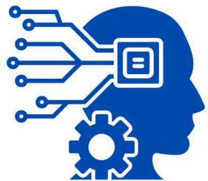
MACHINE LEARNING
